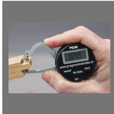
Peak Digital Pipe Thickness Caliper
