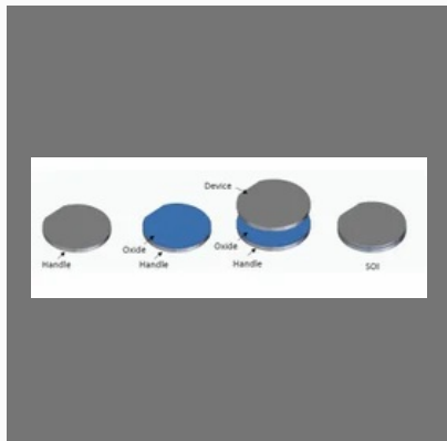
SOI (Silicon on Insulator) Wafer Substrates
