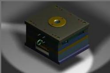
Dowel Block For Tyre Mould
