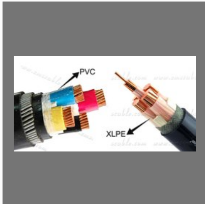
XLPE Cable
