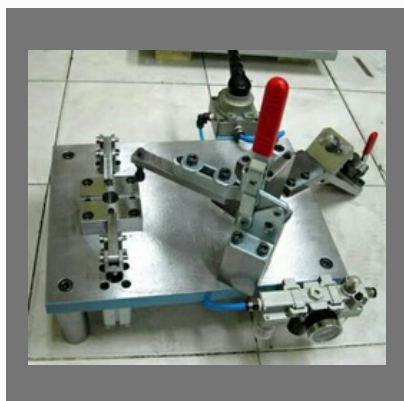
Jig Fixture
