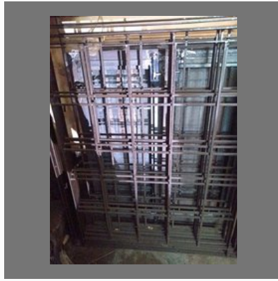
MS Window
