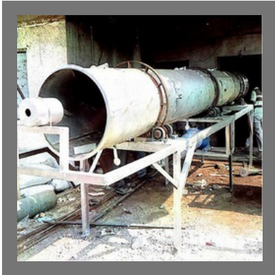
Rotary Dryer Fabrication Service
