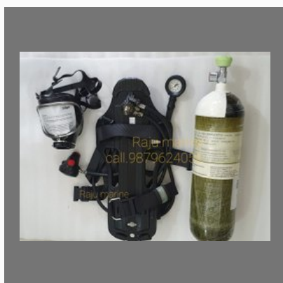
Drager PA 90 Plus Self Contained Breathing Apparatus (SCBA) With Carbon. Cylinder 45 minutes
