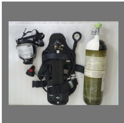
Drager Pa91 Plus . Carbon( Self Contained Breathing Apparatus), For Firefighting,
