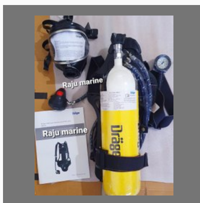
Drager Pa 91 Plus Self Contained Breathing Apparatus (scba) With Carbon Composite Set
