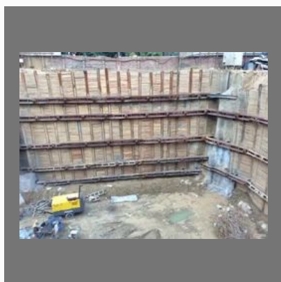
Shoring With Soldier Pile Work in Delhi, Noida, Gurugram, Faridabad, Ghaziabad
