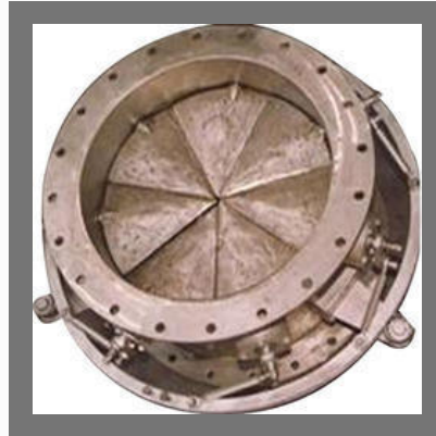
Inlet Guide Vane Damper
