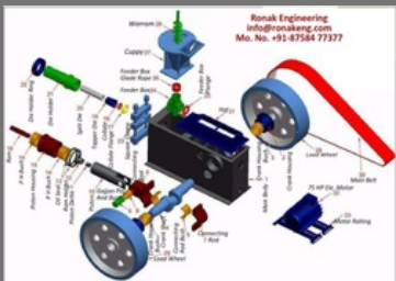
Briquette Machine Spare Parts
