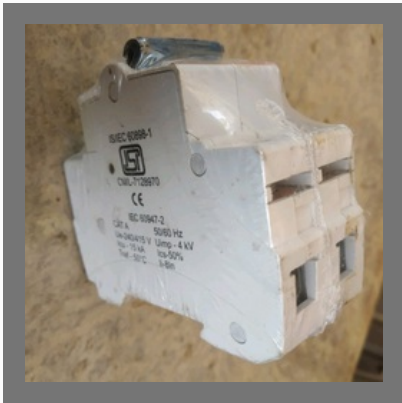
Circuit Breakers
