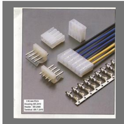
Cable Connectors
