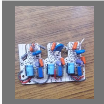
Bulb PCB
