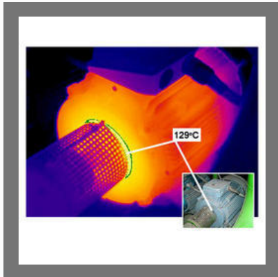
Thermography Services
