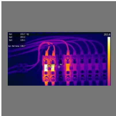
Thermography Survey
