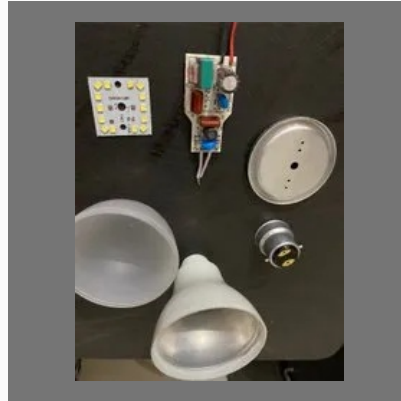
12 W Bulbs
