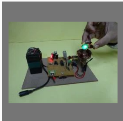
Wireless Power Transmission Project
