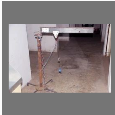
Folding Battery Operated Crane
