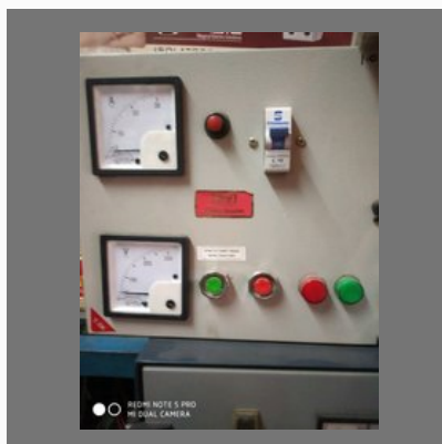
Motor Panel
