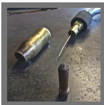
Steel Robotic Welding Machine Nozzle
