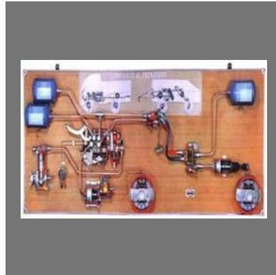
Automotive Hydraulic Pneumatic Braking System
