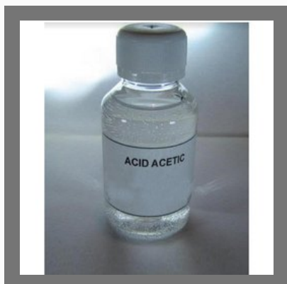
Acetic Acid
