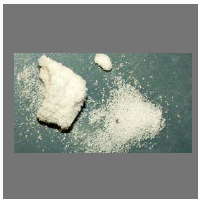
Ammonium chloride
