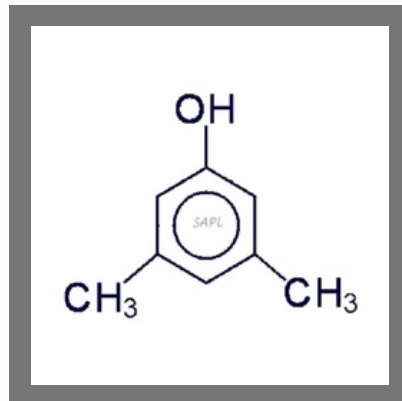
3, 5-Xylenol
