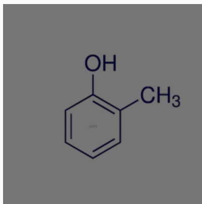
Ortho Cresol
