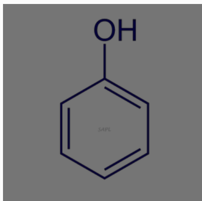
Phenol Chemicals
