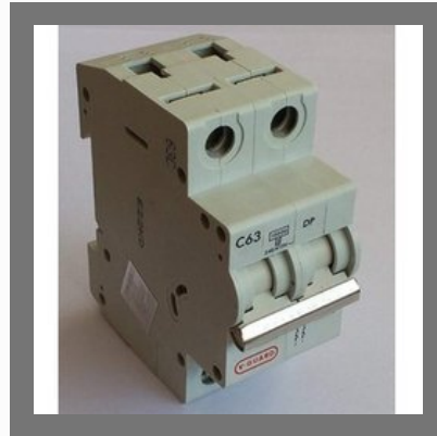
63 A DP V Guard Isolator
