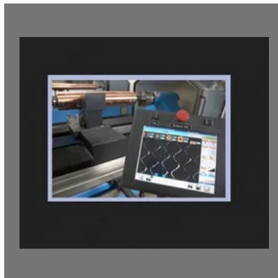
Electro-Mechanically Engraved Rollers
