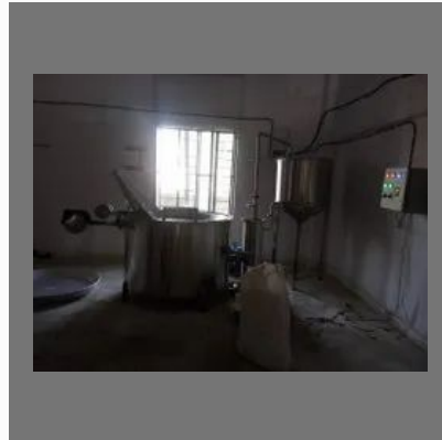
Circular Batch Type Frying System
