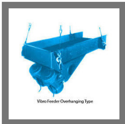
Mechanical Vibro Feeder
