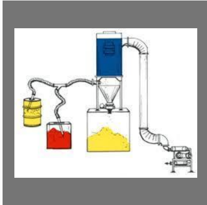
Vacuum Conveying System
