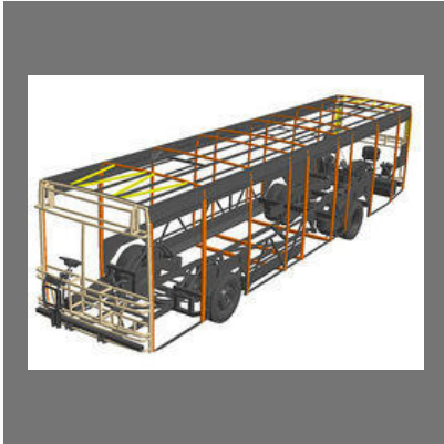
Structural Underframe Bus Body
