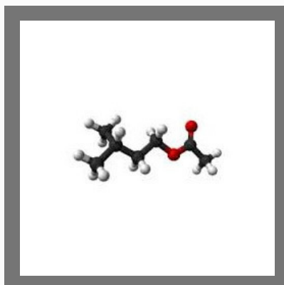
Isoamyl Alcohol
