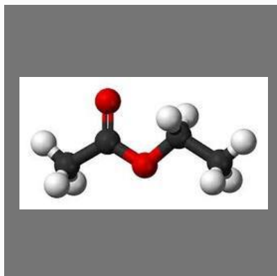
Ethyl Acetate
