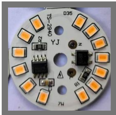
7 Watt COLOR Direct On Board LED SMD PCB
