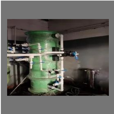
Mix Bed DM Plant
