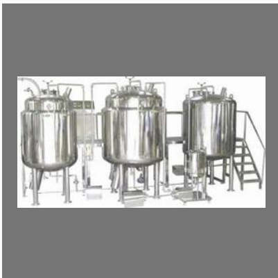
Automatic Oral Liquid Syrup Manufacturing Plant
