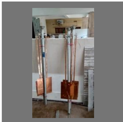
Copper pipe earthing set
