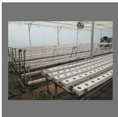
Automatic UPVC Hydroponics Systems, Capacity: Acre
