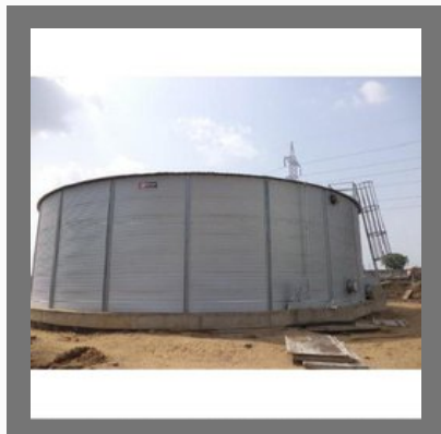
Zinc Alluminium Water Tanks
