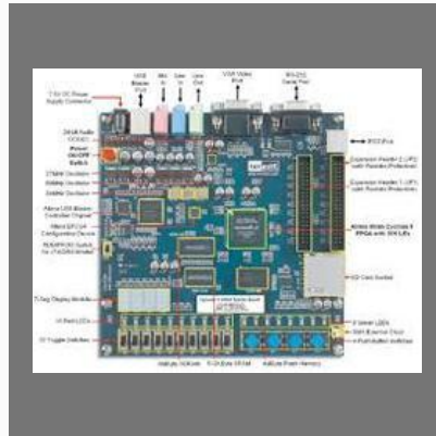
Altera Cyclone 2
