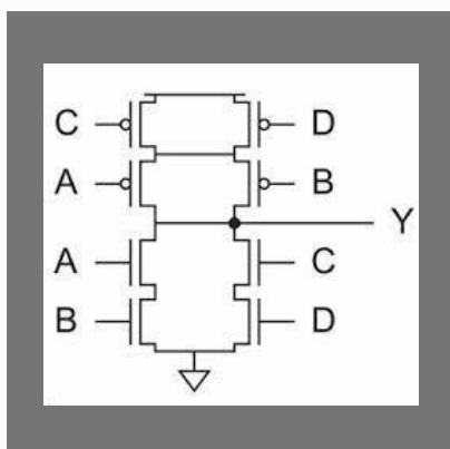
Cmos-logics
