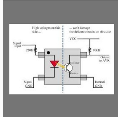
Opto-coupler
