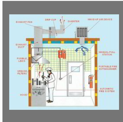
Kitchen Duct
