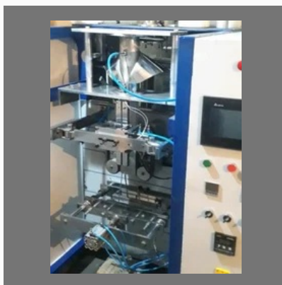
Collar Type Packing Machine
