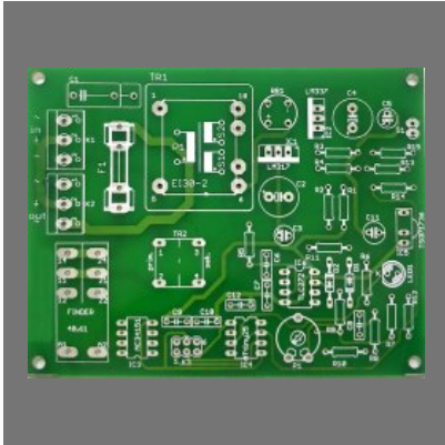
Anti Standby Switch(PCB)
