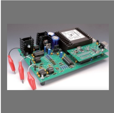
Transistor Curve Tracer(KIT)
