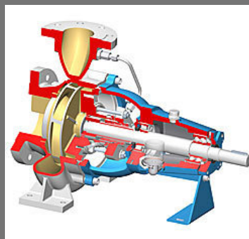
CombiChem Pump
