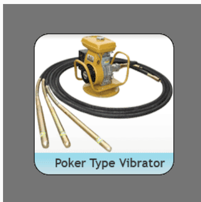
Concrete Vibrator
