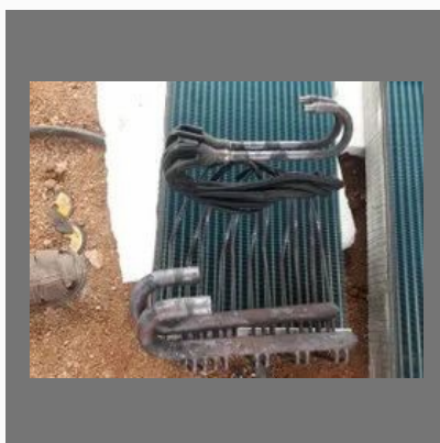
Evaporator Coil
