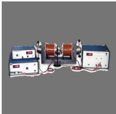
Hall Effect Setup Standard Make, SES
