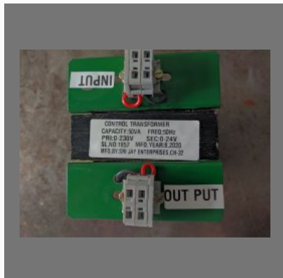
50va control transformer
