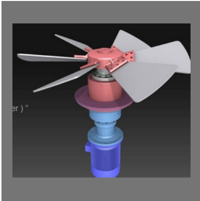
Mechanical Circulator
