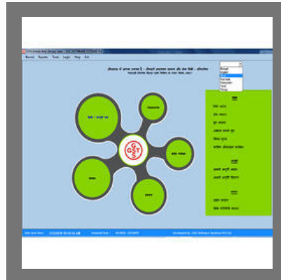
GSTGSS Software
