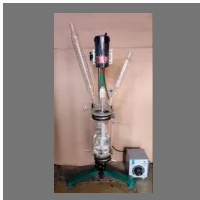
Double Wall Glass Jacketed Reactor
