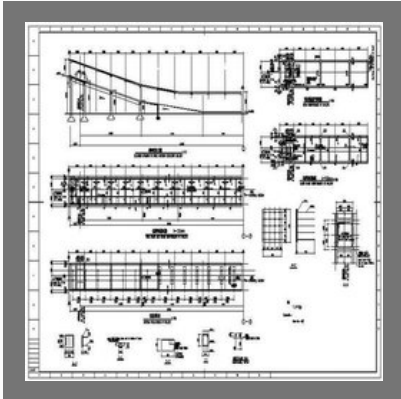
Structural Drawing
