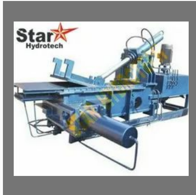
Triple Compression Scrap Baling Machine
