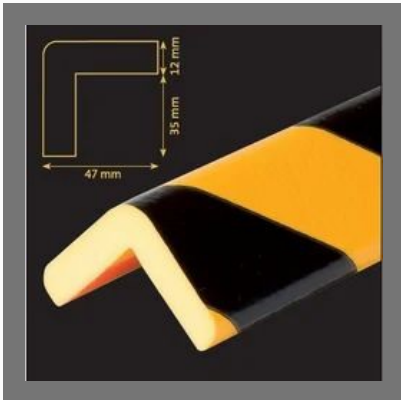
Type H Knuffi Corner Protector Guard
